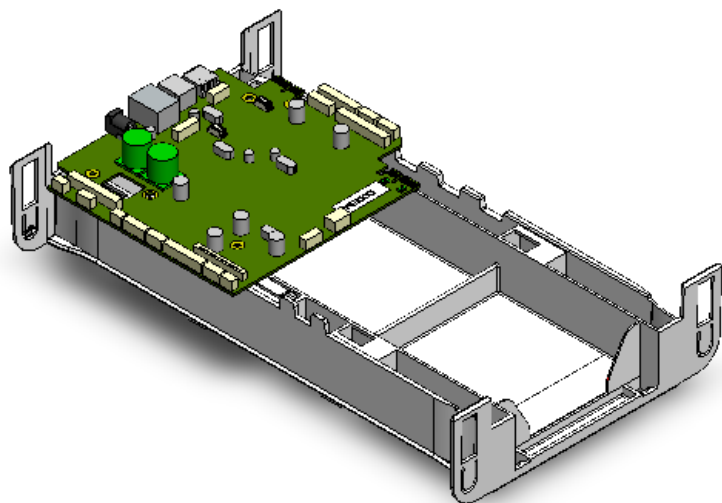
MAIN BOARD : USB ETH USB-HUB S10114
